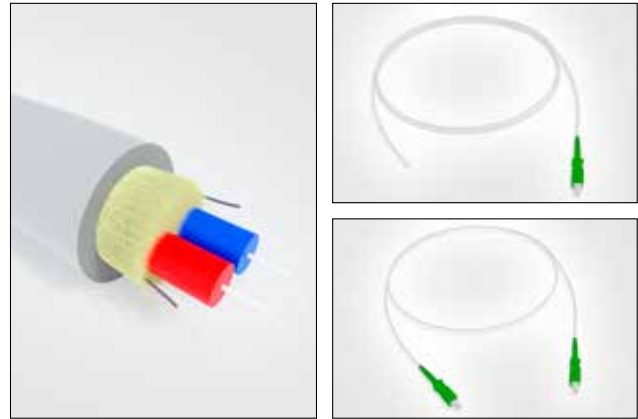
Main image left: 2 fibre bare end cable. Top right: 1 fibre SC / APC SX pigtail. Bottom right: 1 fibre SC / APC SX patch lead.
