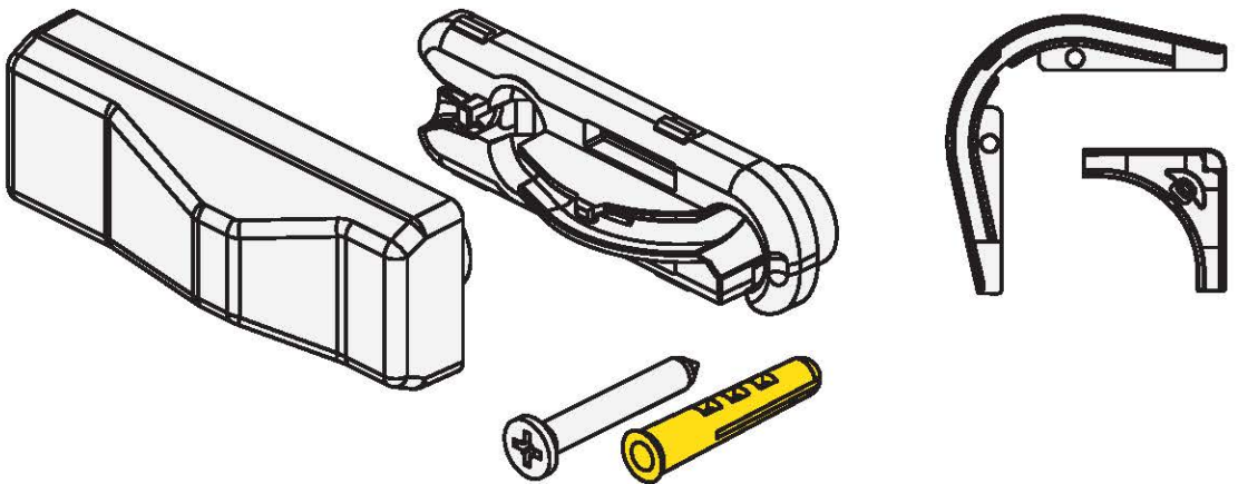
FM-P388-042-00 Cable Management Kit Straight 1.5mm / 3.0mm G657.A2
